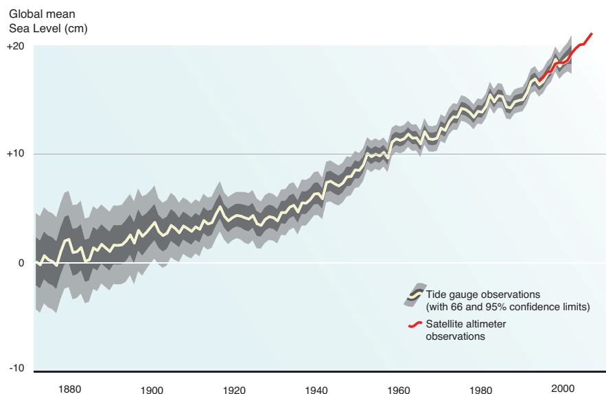
Figure 2 : Rising trend in average sea level
