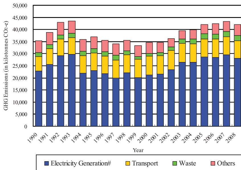
Figure 4 : GHG Emission Trends of Hong Kong from 1990 – 2008
