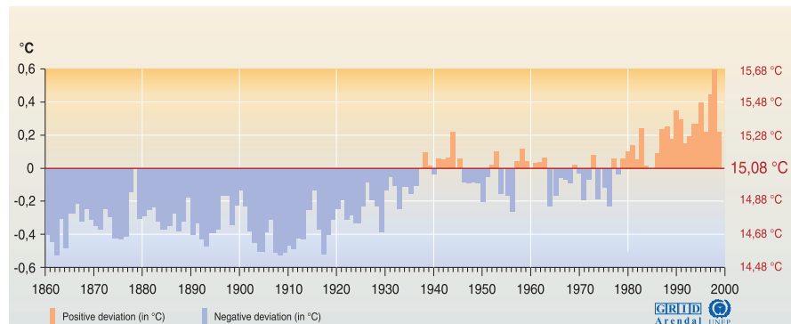
Figure 1 : Increasing trend in average global surface temperature
